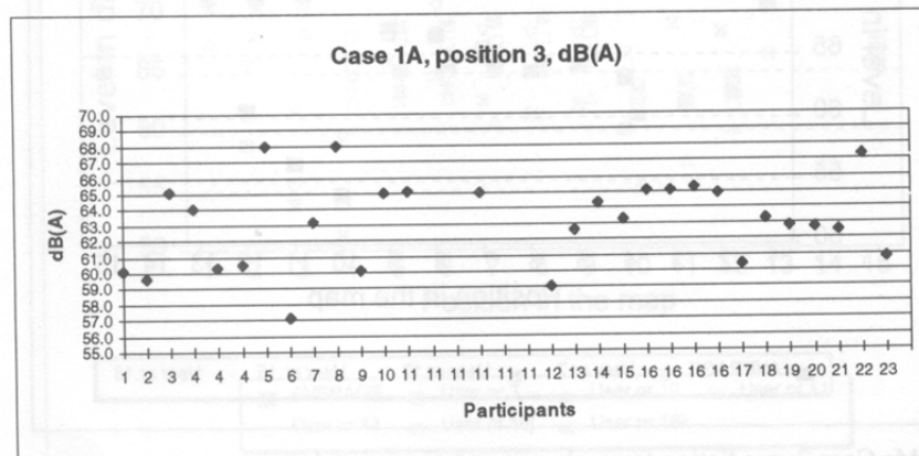
Fig. 19: Lmed = 63.1 dB(A) Lmax - Lmin = 10.9 dB(A) Std.Dev. = 2.69
